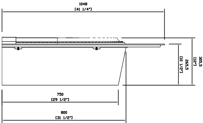
Side Elevation
