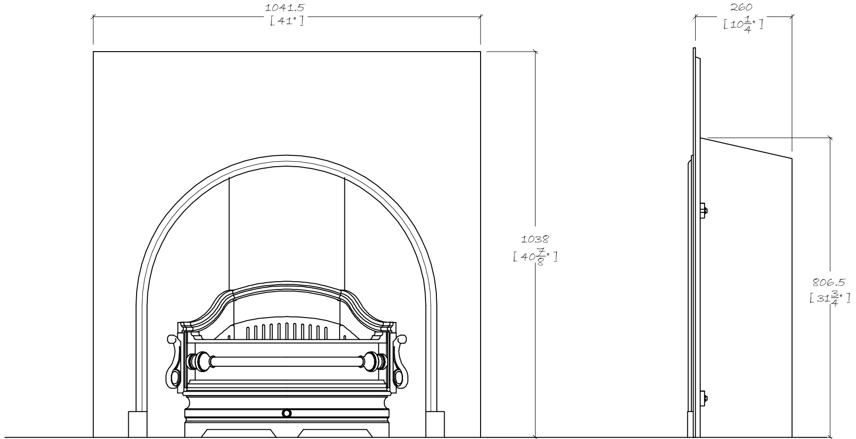
SIDE ELEVATION
